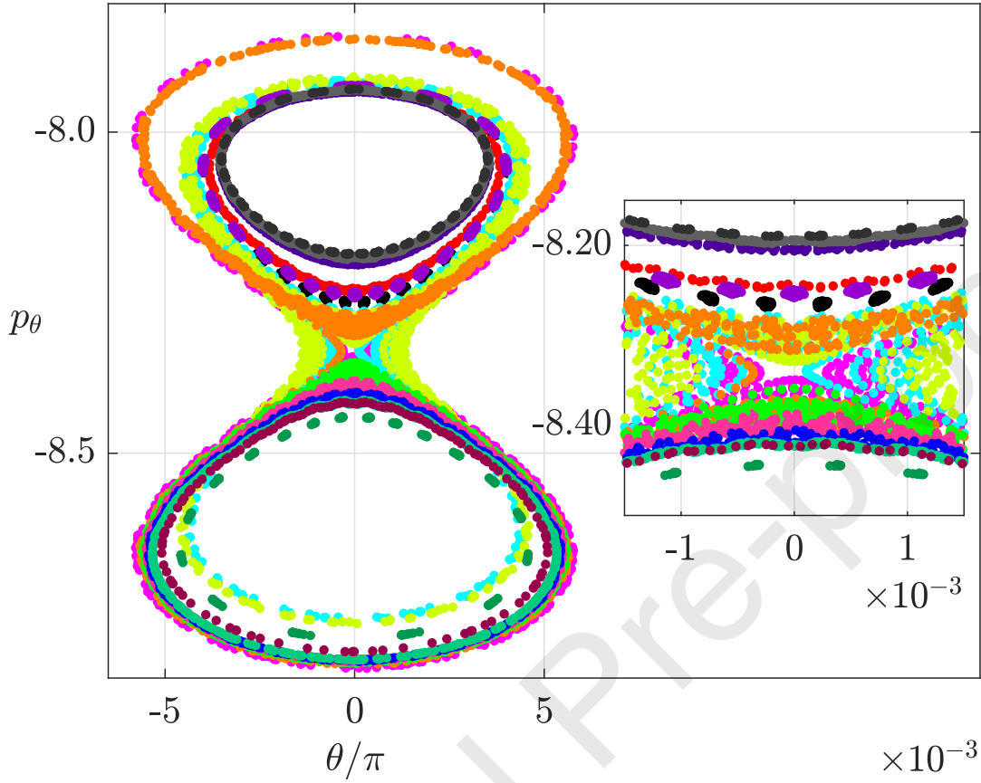
Fig. 6: Poincaré section ( p_r = 0 plane) of trajectories of trapped ions. All trajectories have \mathcal{H}_i \approx 0.062 , but different sets of (r_0, \theta_0, \zeta_0) , each one identified by a different color.
