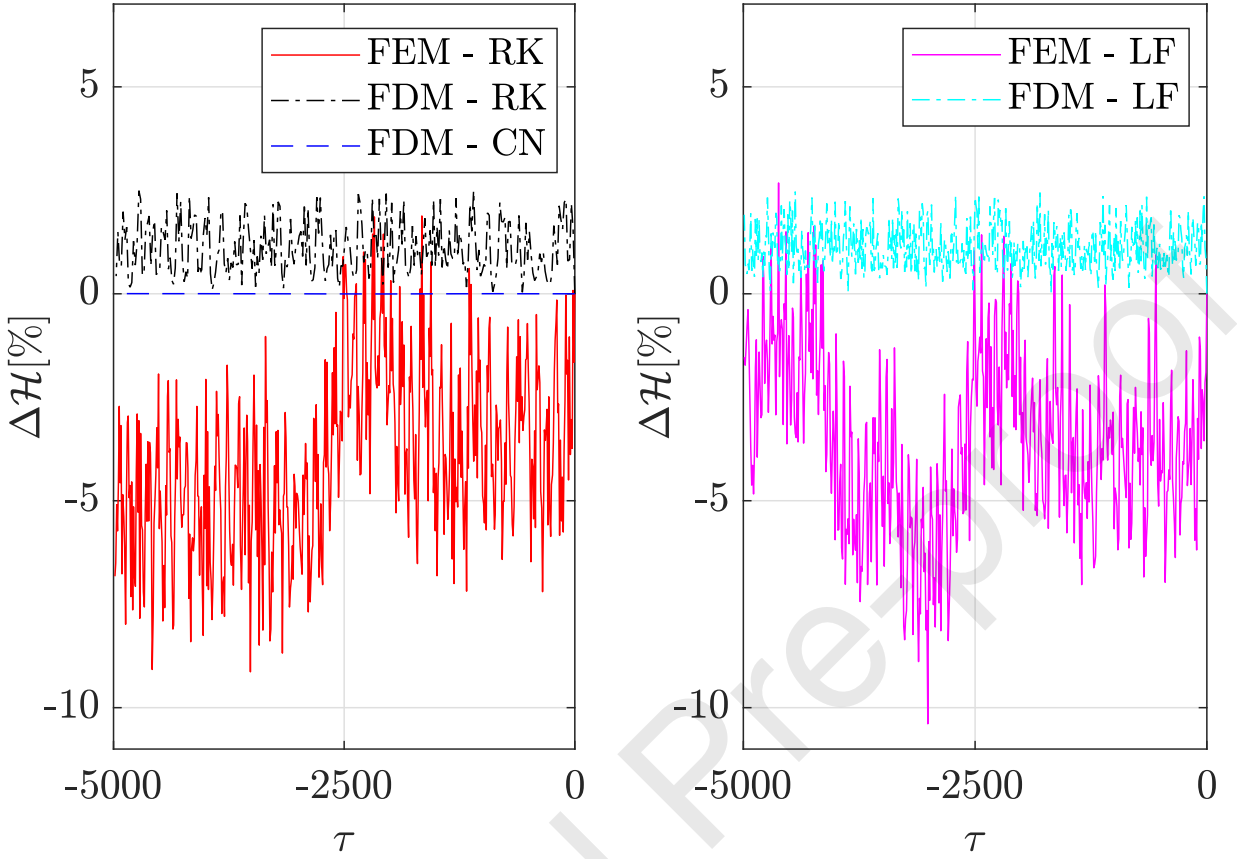
Fig. 4: Evolution of \Delta\mathcal{H} = [\mathcal{H}(\tau) - \mathcal{H}(0)] \times 100/\mathcal{H}_0 for a trapped ion moving around an elliptical probe ( e_p = 0.95 ).
