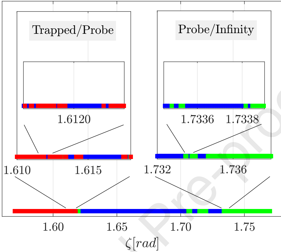
Fig. 7: Structure of the ion distribution function at (x, y) = (3.54, 0) with \mathcal{H}_i \approx 0.062 . Research data and post-processing scripts can be found at [dataset][33].
