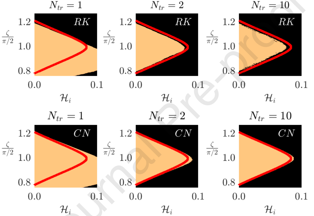
Fig. 5: Distribution function at (x, y) = (3.05, 0) in the \mathcal{H}_i - \zeta plane for different values of N_{tr} obtained with the RK (top) and CN (bottom) solvers. Orange and black regions correspond to initial conditions yielding trajectories that are trapped and hit the unperturbed plasma boundary of the computational domain, respectively. The red line is the boundary obtained with the solver of Ref. [27]. Research data and post-processing scripts are available at the [dataset] [33].
